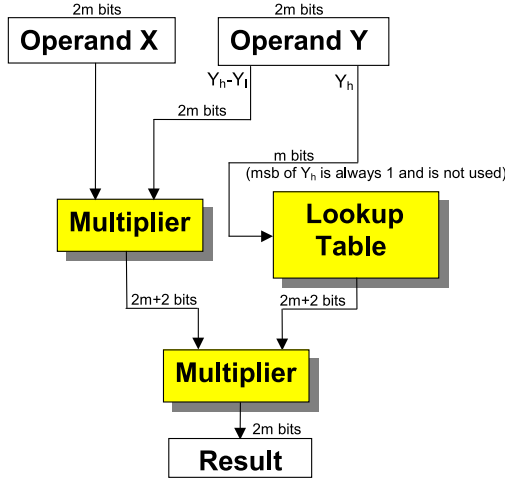
Figure 1: Basic Algorithm
