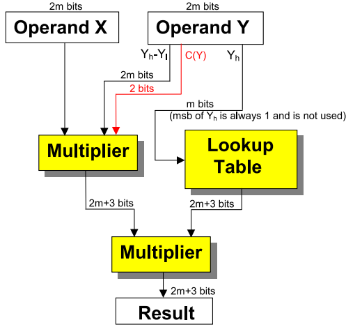
Figure 3: Error Compensation
